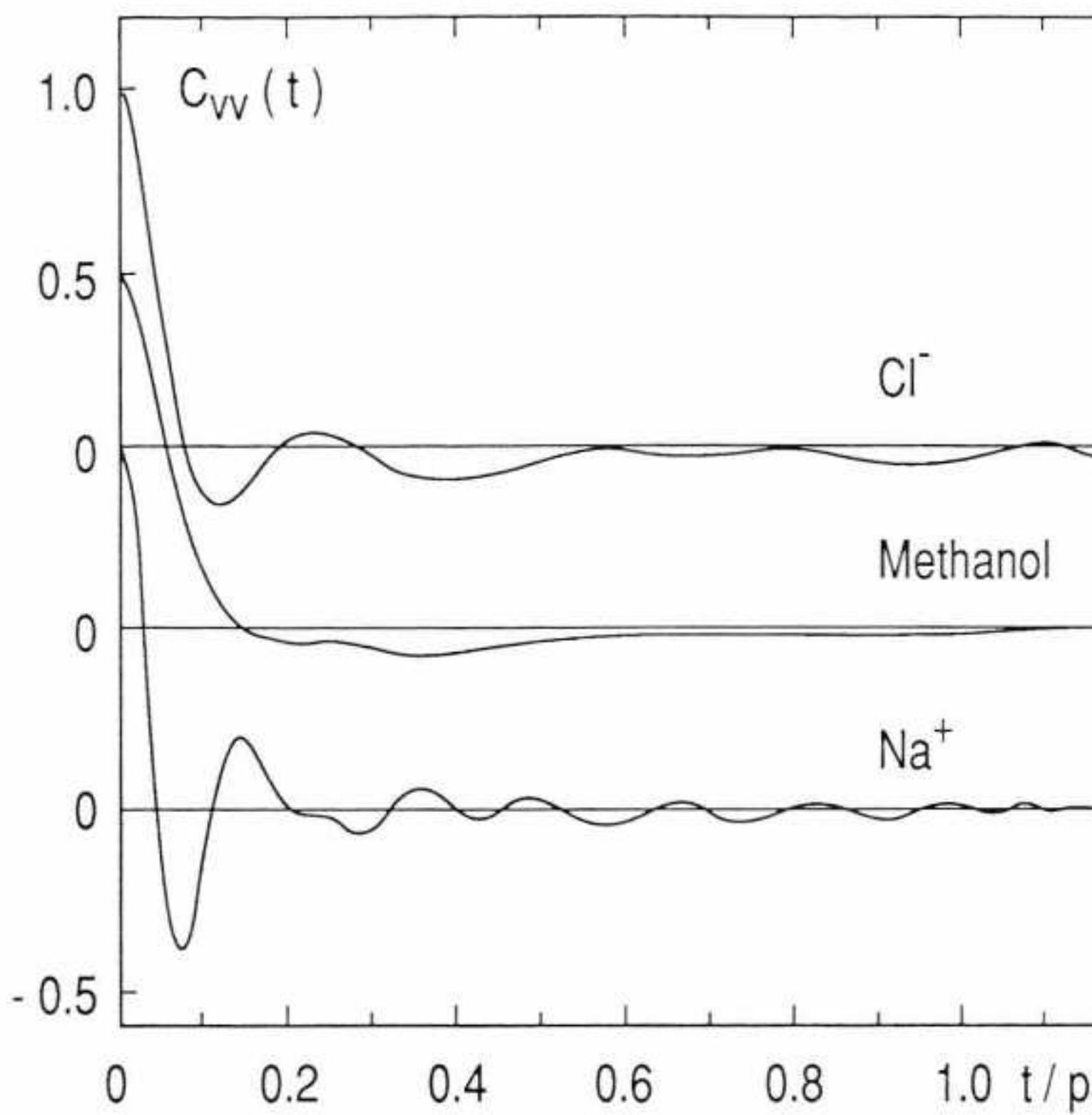
Fig. 11. Normalized velocity autocorrelation function
