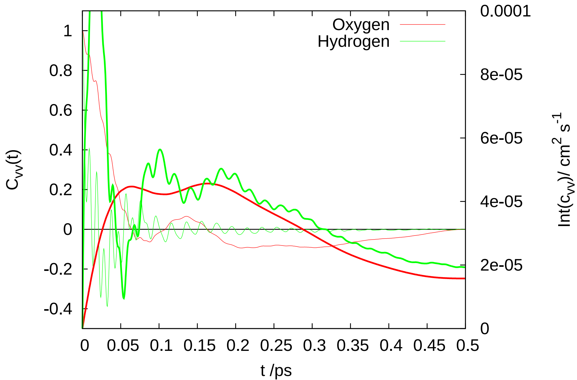
C_{VV} and integrals
